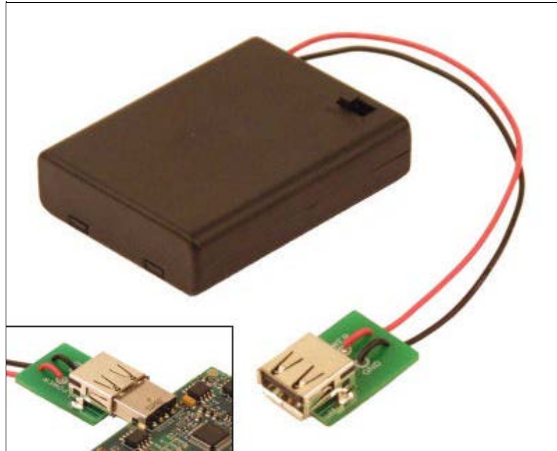
Battery Backup for C55xx eZdsp USB Stick
