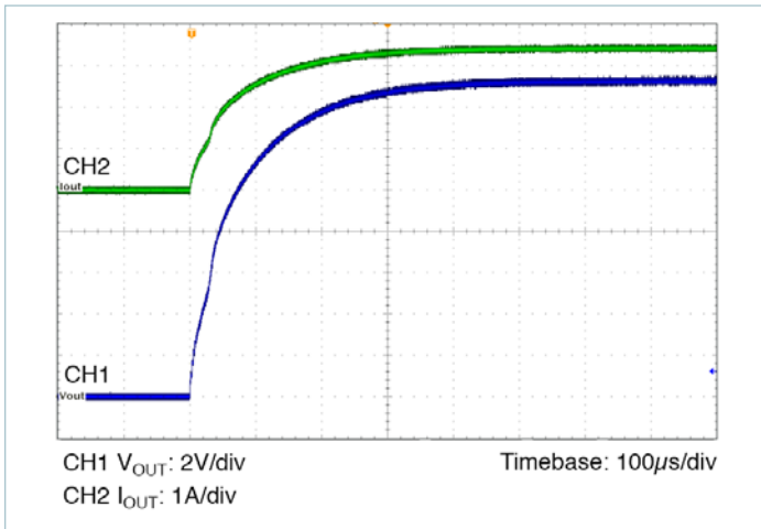
Figure 37 — Start Up, C_{REF} = 0 ( V_{IN} = 50V , I_{OUT} = 3.3A , C_{OUT} = 6 \times 2.2\mu F X7R Ceramic)
