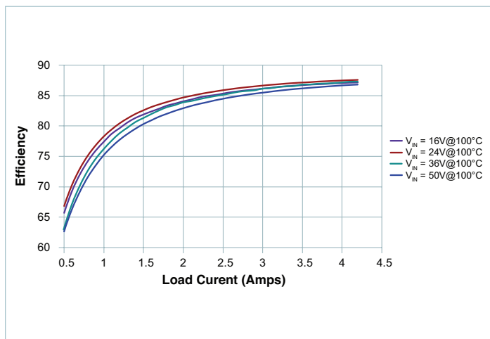
Figure 21 — Conversion Efficiency
