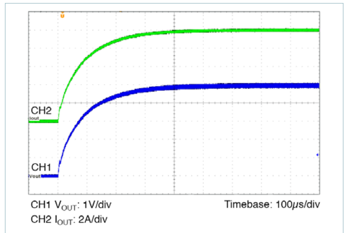
Figure 16 — Start Up, C_{REF} = 0 ( V_{IN} = 28\text{V} , I_{OUT} = 10\text{A} , CR, C_{OUT} = 6 \times 10\mu\text{F} X7R Ceramic)
