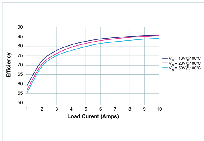
Figure 1 — Conversion Efficiency
