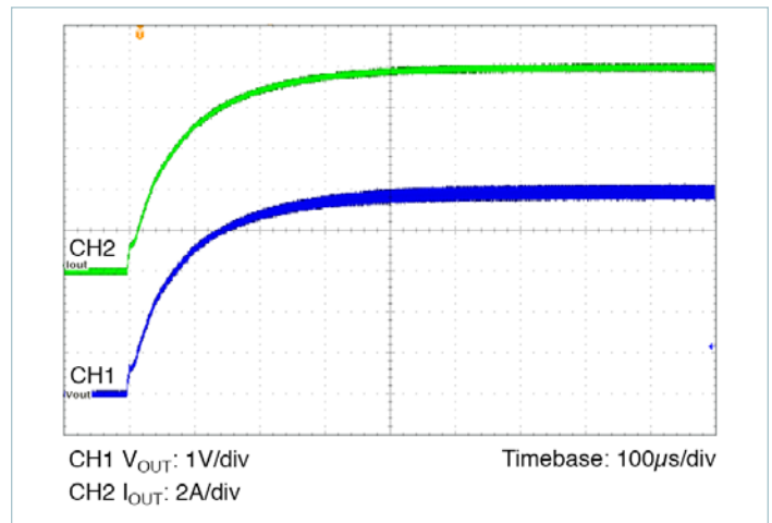
Figure 15 — Start Up, C_{REF} = 0 ( V_{IN} = 16\text{V} , I_{OUT} = 10\text{A} , CR, C_{OUT} = 6 \times 10\mu\text{F} X7R Ceramic)
