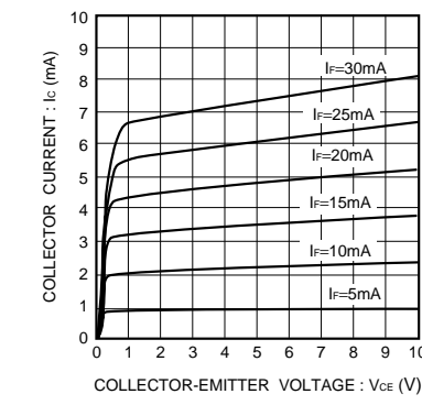
Fig.10 Output characteristics
